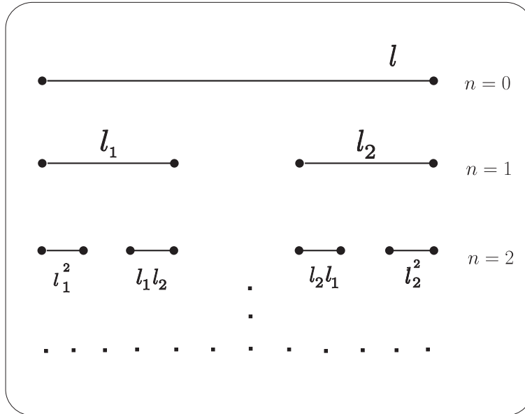
Fig. 1. Two-scale Cantor set.
