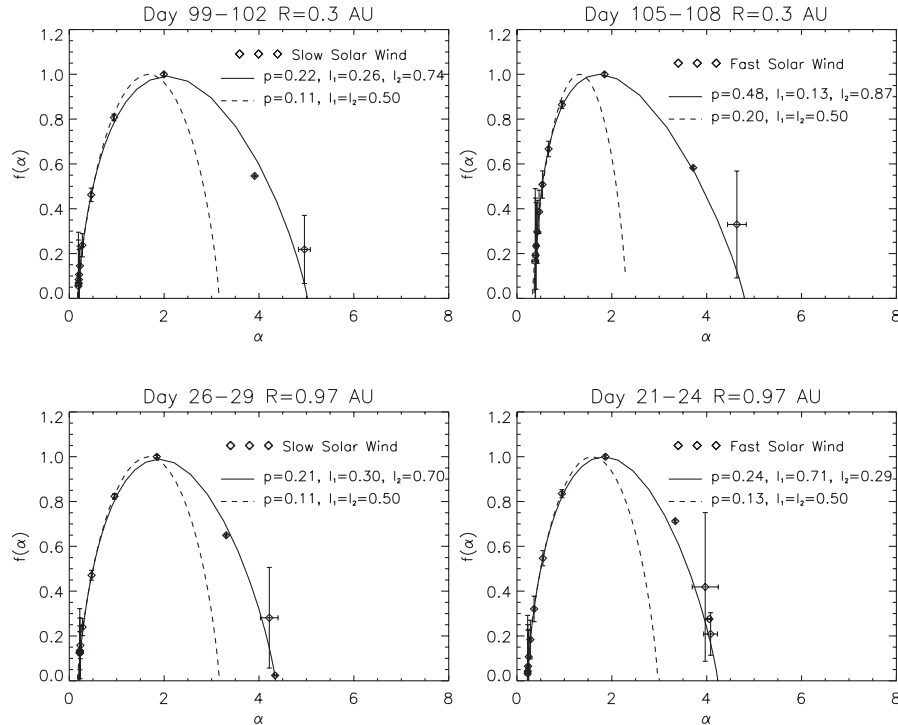
Fig. 2. The singularity spectrum f(\alpha) as a function of \alpha . The values of for one-dimensional turbulence are calculated for the generalized two-scale (continuous lines) and the usual one-scale (dashed lines) p -model and fitted using the v_x velocity components (diamonds) for the slow (a) and (c) and fast (b) and (d) solar wind streams at distances of 0.3 AU and 0.97 AU, correspondingly.
