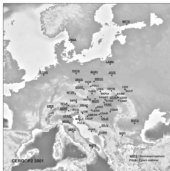
Fig. 4. CERGOP-2 2001 network
