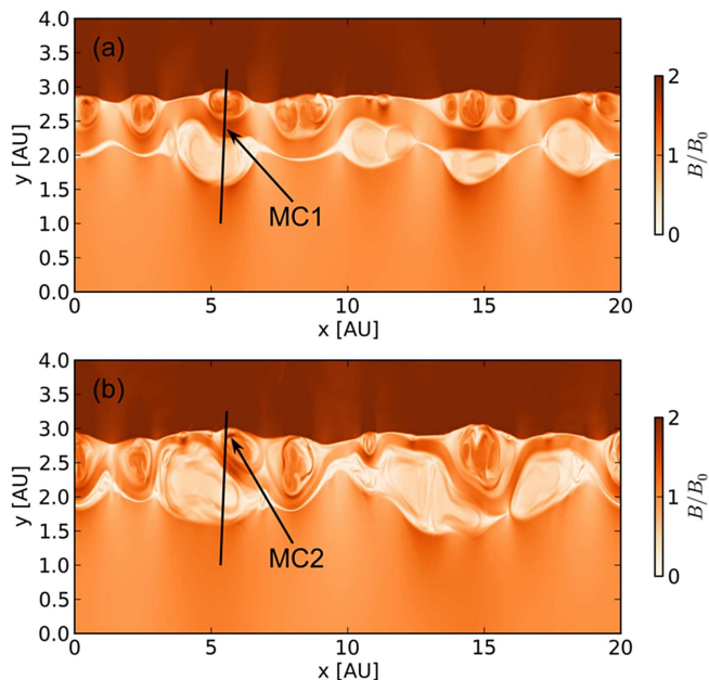
FIG. 4.— Development of magnetic islands and magnetic compressions in the simulation for (a) t/T_0 = 23.0 and (b) t/T_0 = 26.1 . The magnetic islands can be seen quite clearly in panel (a) as local thickenings of the current sheets SCS1 ( y \approx 2 , low values of B/B_0 ) and SCS2 ( y \approx 2.75 , sharp gradient of B/B_0 ). The non-labeled black line shows the x - y plane projection of the virtual spacecraft trajectory for which profiles from Figure 3 are obtained. Locations of the magnetic compressions MC1 and MC2 from Figure 3 are shown by arrows. The aspect ratio of the plot has been altered to better visualize details.
