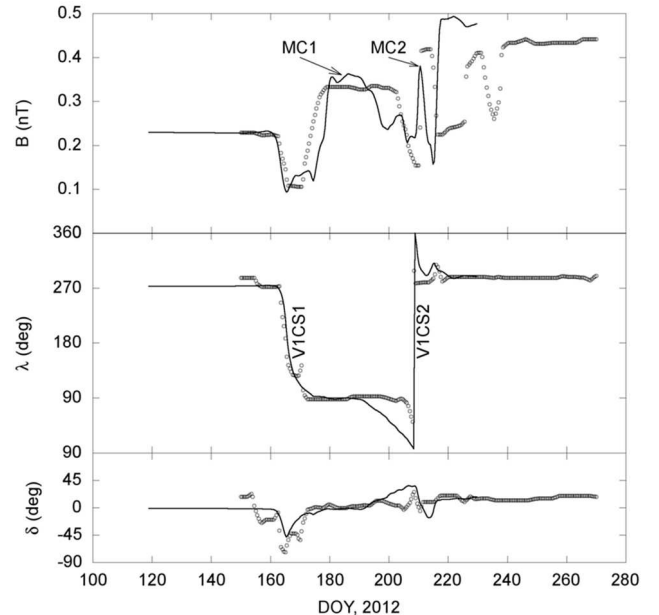
FIG. 3.— Comparison of the profiles of the magnetic field strength B , and the \lambda and \delta angles measured by the V1 spacecraft (circles) with corresponding profiles (properly shifted and rescaled) obtained for a virtual spacecraft moving in the simulation box (solid line).
