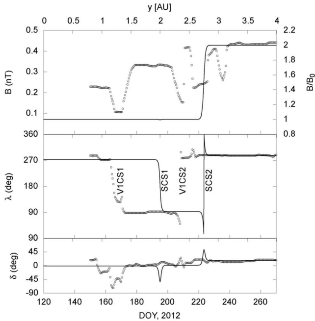
FIG. 1.— Profiles of the magnetic field strength B , and the angles \lambda and \delta measured by the V1 spacecraft (circles, left vertical and bottom horizontal axes). The solid line shows the profiles set up using the initial condition along the y -axis in our simulation (right vertical and top horizontal axes).
