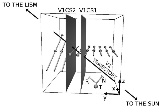
FIG. 2.— Orientation of the simulation frame xyz with respect to the RTN frame, the current sheets V1CS1 and V1CS2 (normal to the y -axis), and the V1 trajectory (along the R -axis approximately). The direction of the magnetic field lines is shown by non-labeled gray arrows inside the box, the vector direction changes at the current sheets V1CS1 and V1CS2.
