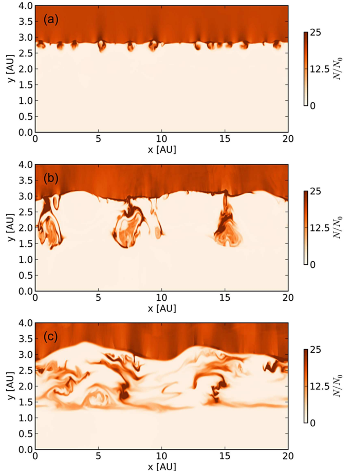
FIG. 5.— Development of the density intrusions caused by the transport of the dense LISM plasma to the IHS for (a) t/T_0 = 20 , (b) t/T_0 = 35 , and (c) t/T_0 = 60 . The aspect ratio of the plot has been altered to better visualize details.
